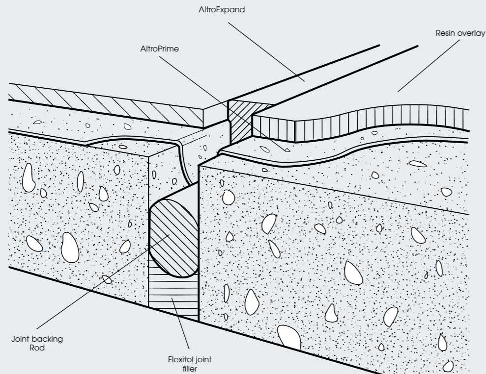
Altro resin overlayment transition joint detail
